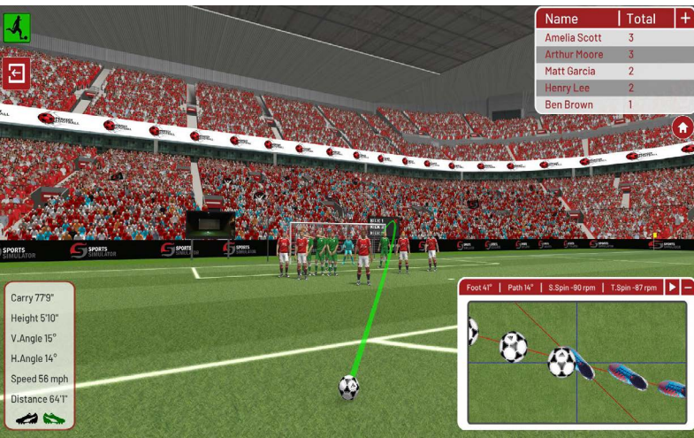
RIGHT FOOT SHOT ANALYSIS - GOAL
